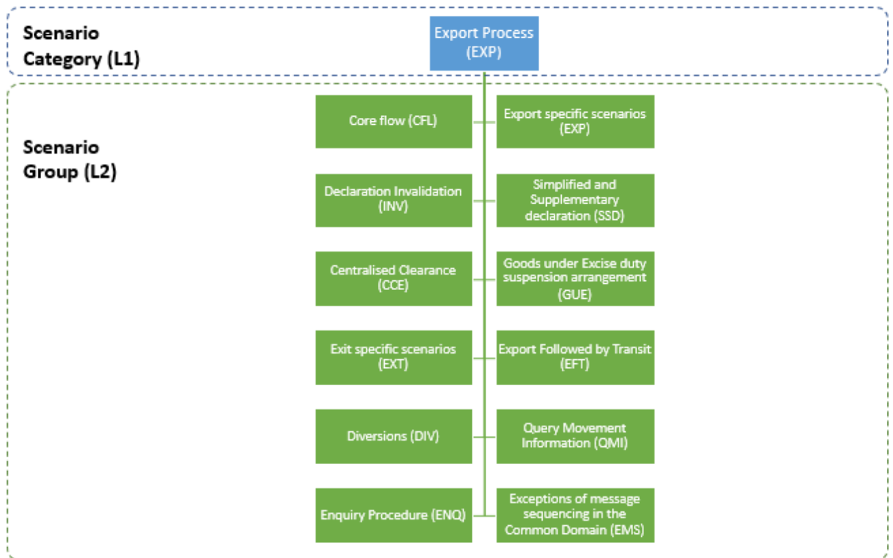
Figure 6: Export Process
